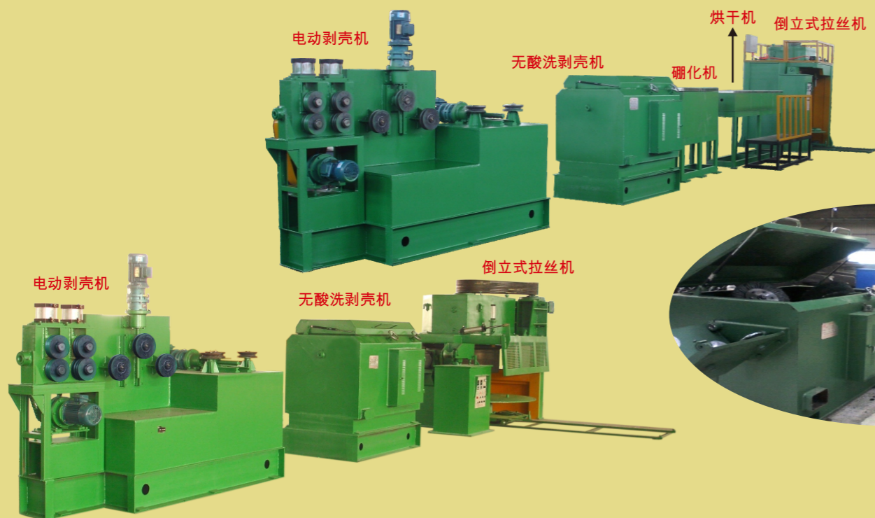
▲ LDD600-LDD1200型倒立式拉丝机+ BPJ6/30型无酸洗剥壳机+ DDBKJ200(300)型双向电动剥壳机组合组(硼化机组) LDD600-LDD1200 handstand type drawing machine +BPJ6/30 descaling machine+DDBKJ200(300) two-ways electronic descaling machine
