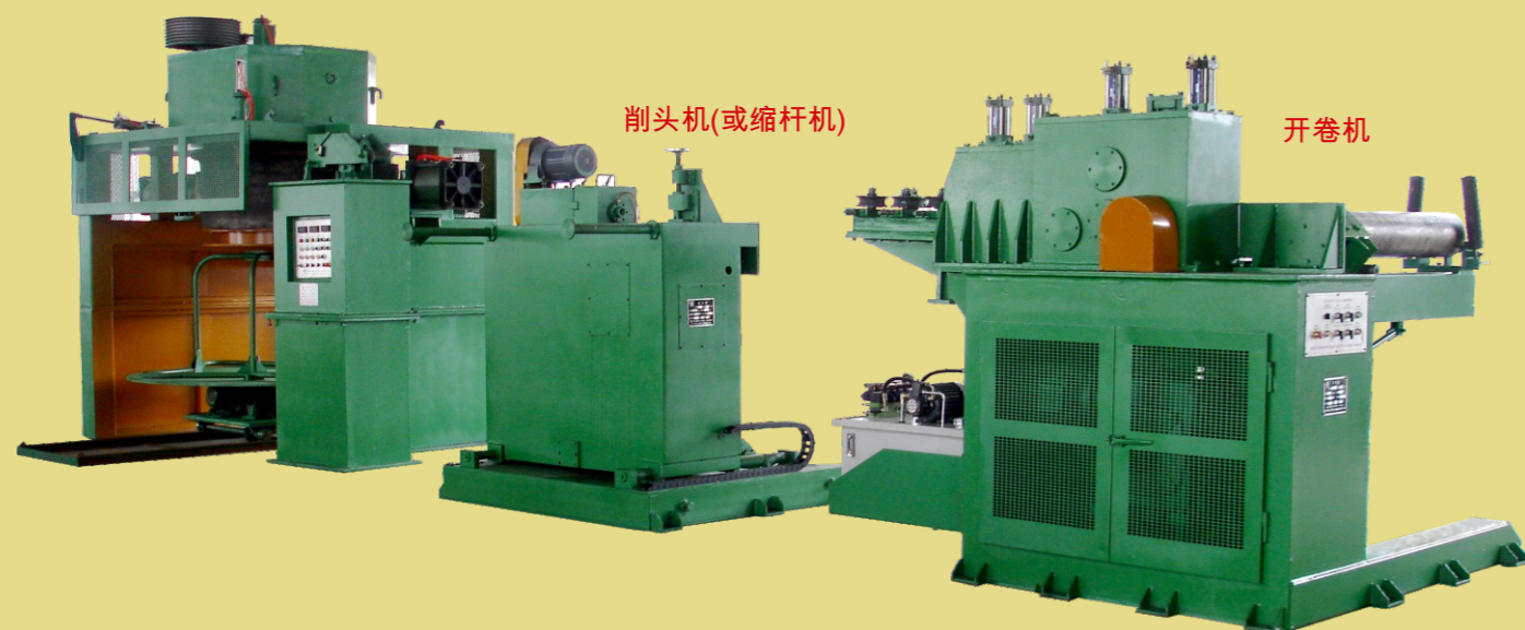
▲ DD1400(LDD1200)倒立式拉丝机+ XTJ40(XTJ30)削头机或液压缩杆机+ KJJ40 ( 30 ) 型开卷送线机组合机组 LDD1400(LDD1200)handstand type drawing +XTJ40(XTJ30) shuck head machine or hydraulic Shrink machine+KJJ40(30) uncoiler
