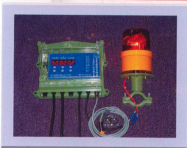
振动送料机电眼控制器 Vibrant feeding machine of electric-eyed controller
